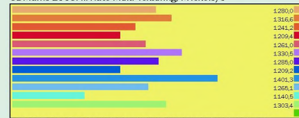
Gun Metal Benchmark 2 (640x480), fps
