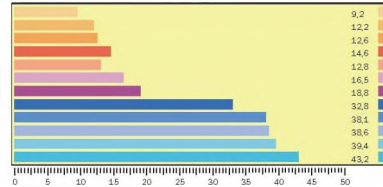
3DMark 03 GT4 - Mother Nature, fps
