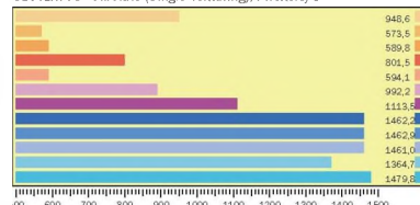
3DMark 03 - Fill Rate (Multi-Texturing), MTexels/s
