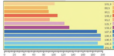
3DMark 03 GT2 - Battle of Proxycon, fps
