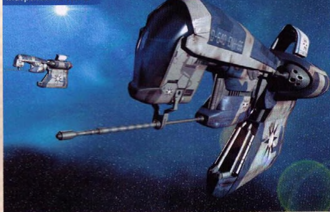
Independence War 2
