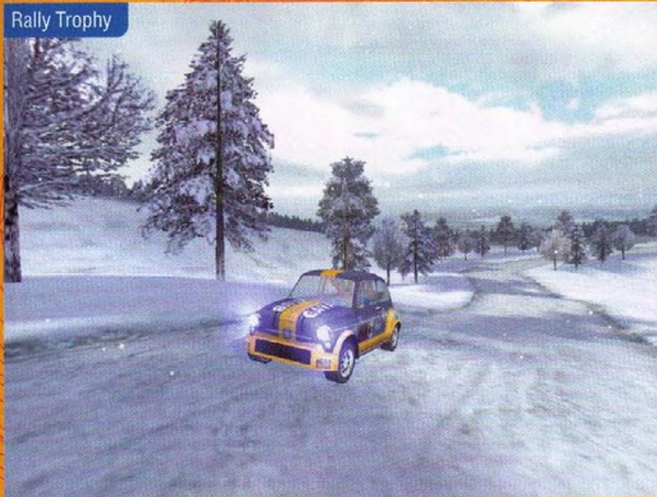
Rally Trophy
