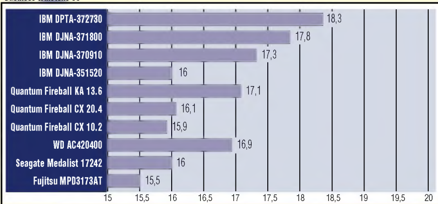
Business Winstone 99
