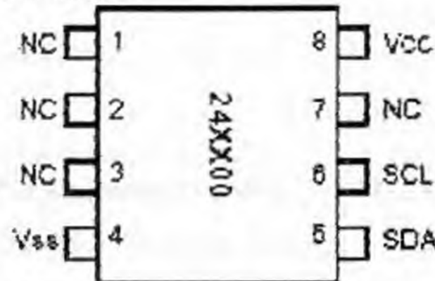
8-PIN TSSOP
